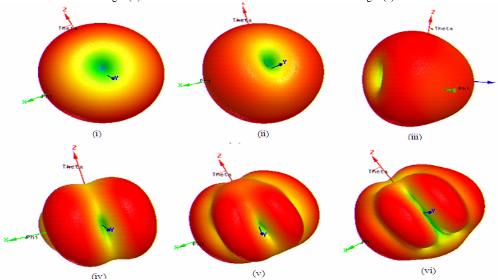
Fig. 1(f) 3D Radiation Plots at (i) 3.1 GHz, (ii) 5 GHz, (iii) 8 GHz, (iv) 9GHz, (v) 10.6 GHz and (vi) 11.2GHz
