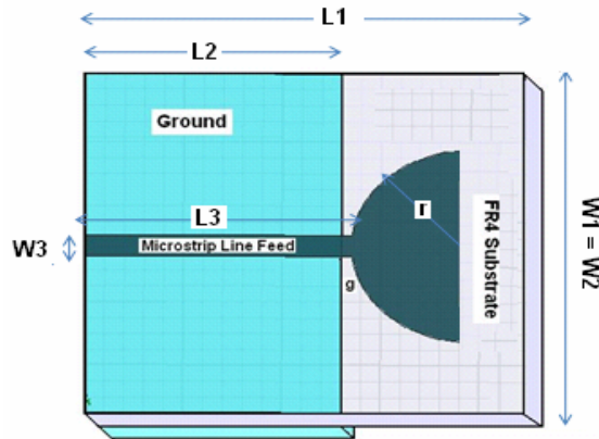
Fig. 1(a) Geometry of Semi-circular UWB Antenna
