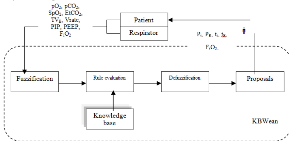
Figure 5: The Fuzzy KBWean control process
